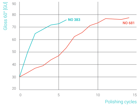
Gloss-cycle-chart of NABALOX® NO 681 and NO 383
